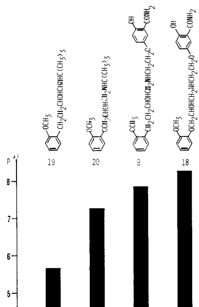
Figure 2. \beta -Blocking potency in vitro in relation to some characteristic structural parameters of the side chain. Footnote a: p = negative logarithm of concentrations of the compounds exerting 50% attenuation of isoproterenol-induced tachycardia.
